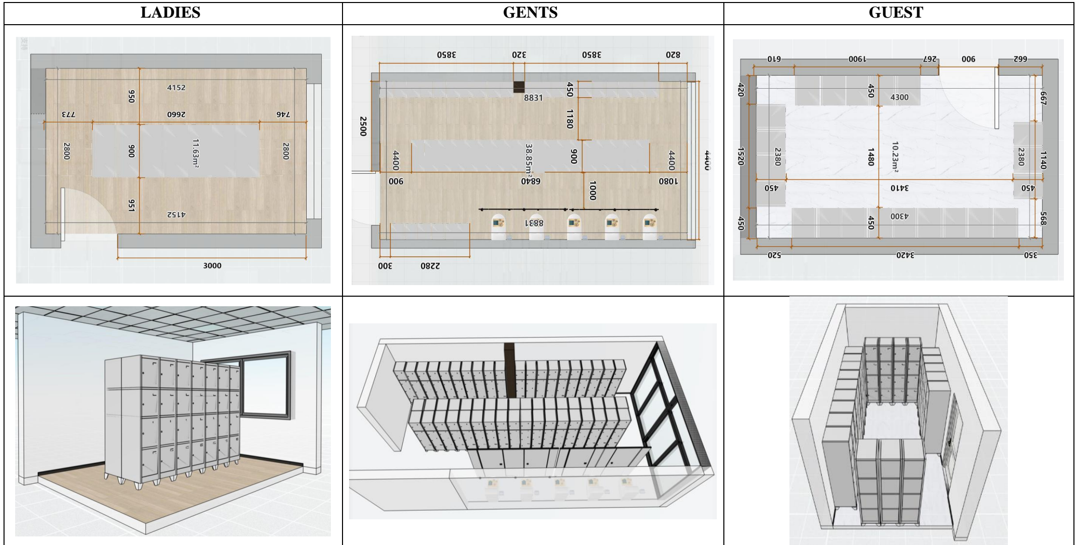
Fig 2: Planned layout of the locker rooms in each section of the QIT
